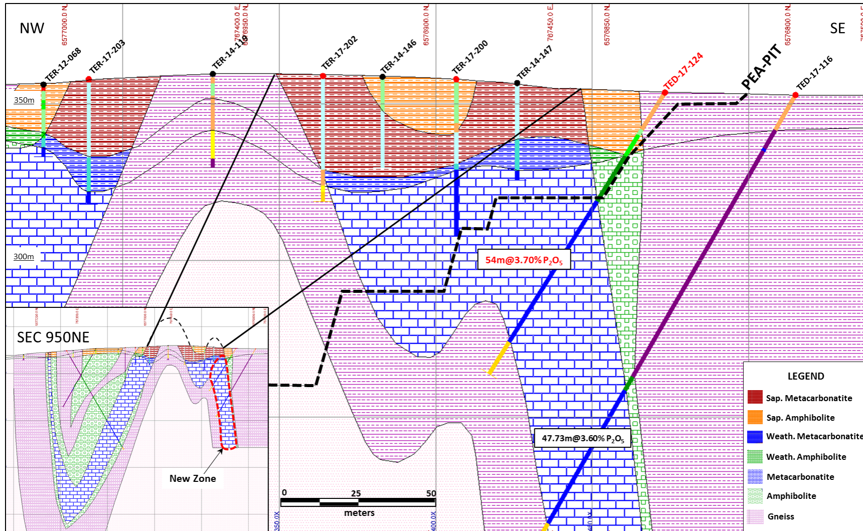
Figure 2: Drilling section 950NE of the Três Estradas Deposit, showing the new southeast zone and one of the highlighted drill results of TED-17-124, which returned recently and confirmed the model of the new zone. Note that the bulk of the new carbonatite drilled in this section is beyond the previous pit model.
